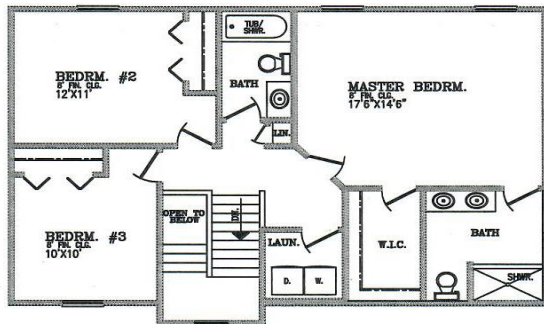
SECOND FLOOR PLAN 3 - BEDROOM
