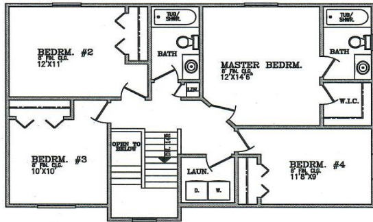
SECOND FLOOR PLAN 4 - BEDROOM
